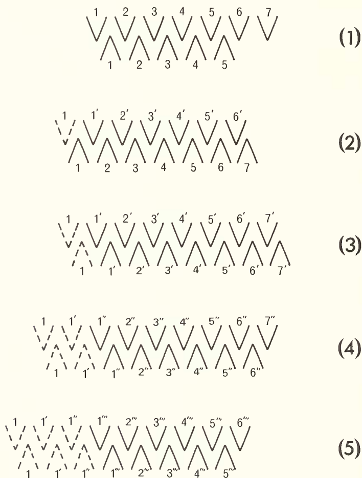
TEXT-FIG. 4. Procolophon trigoniceps . Model of molar succession. See text for explanation. A system of dashes is used to indicate that numbered teeth are not the same teeth as those occupying the same position in previous stages.
